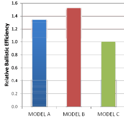
Figure 6. Ballistic Efficiency
