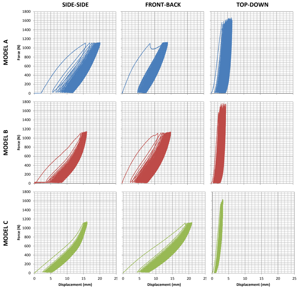
Figure 8. Force-Displacement (60 Cycles)
