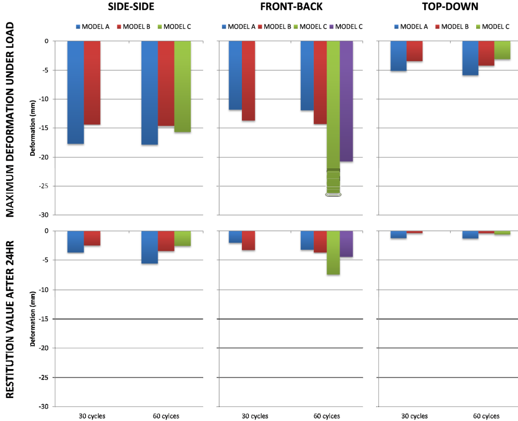
Figure 7. Helmet Deformation
