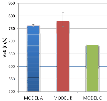
Figure 5. Ballistic Limit
