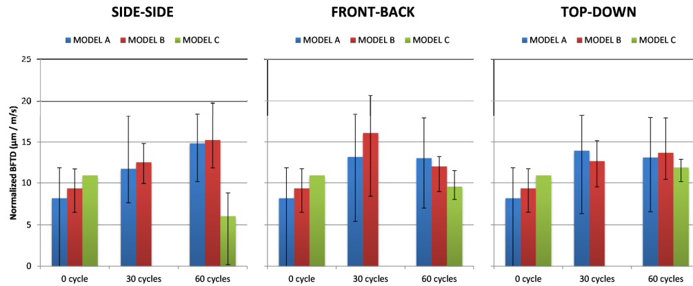
Figure 9. Normalized BFTD
