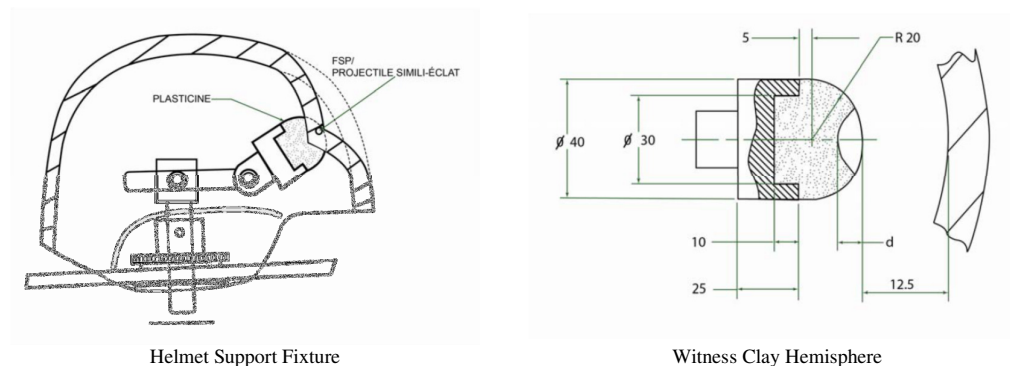
Figure 2. Backface Transient Deformation Test Setup
